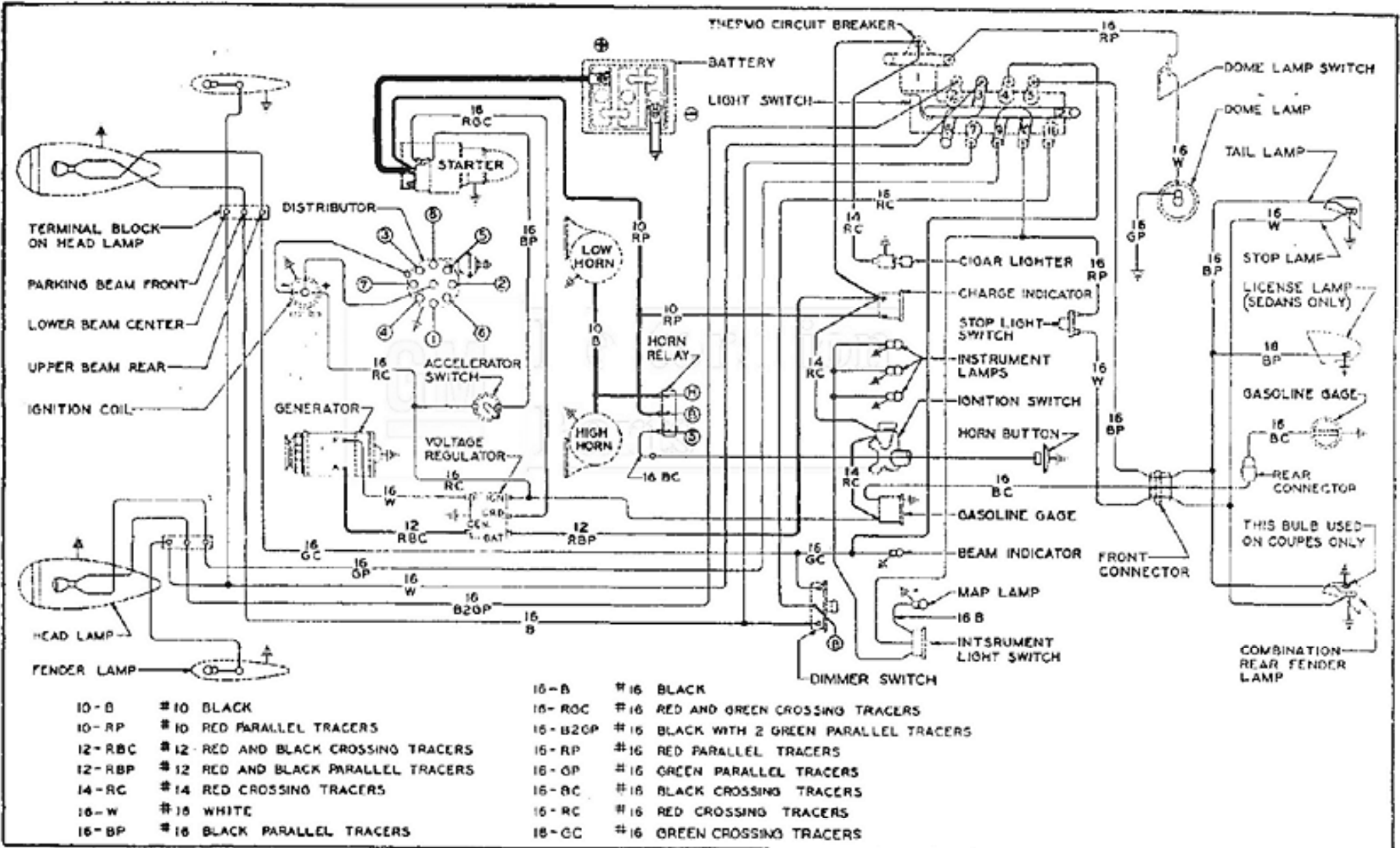
Fig. 12-61. Wiring Diagram—Series 40
